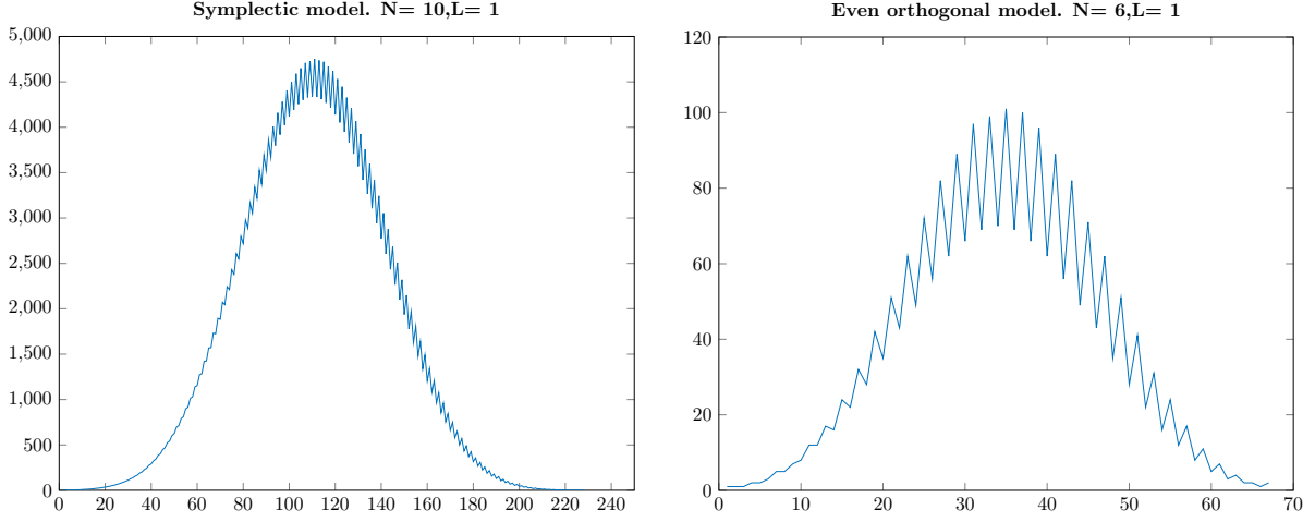
FIGURE 2. For each n in the x axis, the y axis shows the coefficient of the monomial q^{n/2} in Z_{Sp(20)}^{(L=1,m=0)} (left) and Z_{O(12)}^{(L=1,m=0)} (right).
